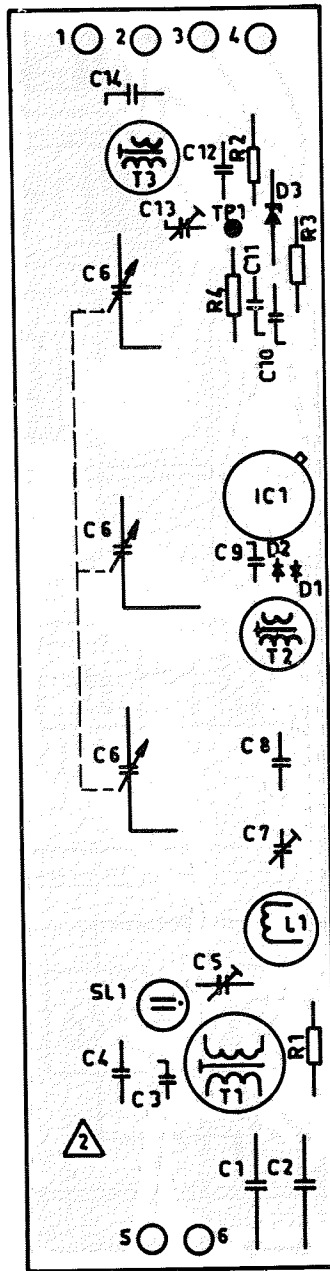
PRINTED CIRCUIT BOARD VIEWED FROM COMPONENT SIDE
