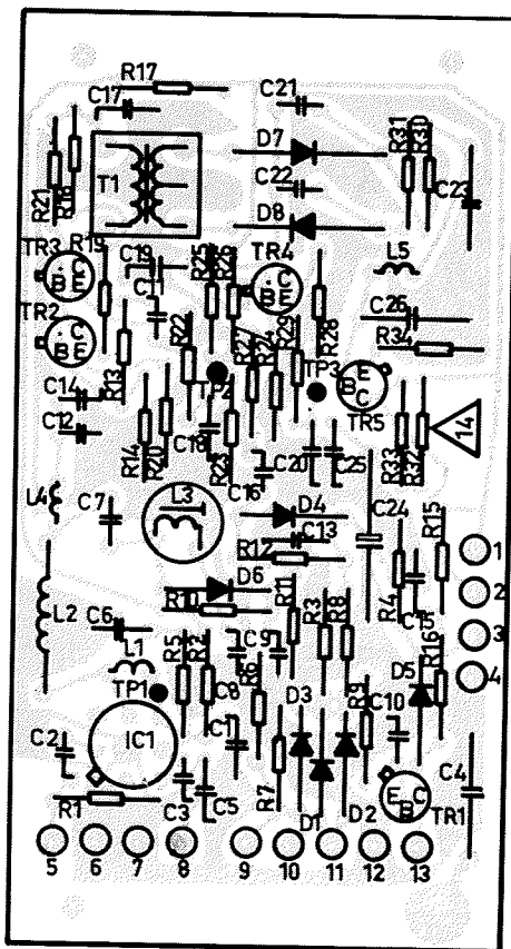
PRINTED CIRCUIT BOARD VIEWED FROM COMPONENT SIDE
