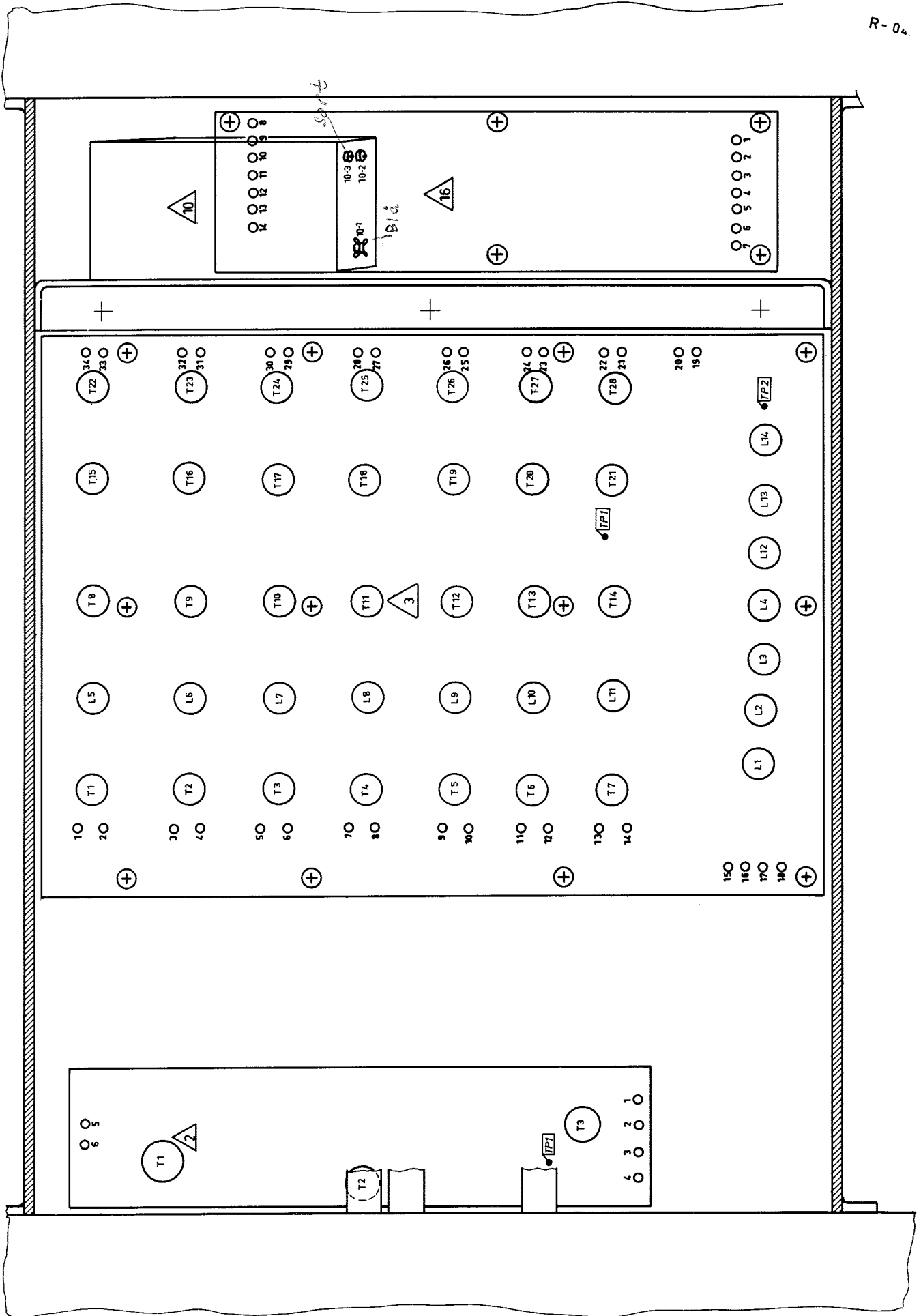
R-0402 - 1 CIRCUIT BOARD LOCATION PLAN BOTTOM COMPARTMENT
