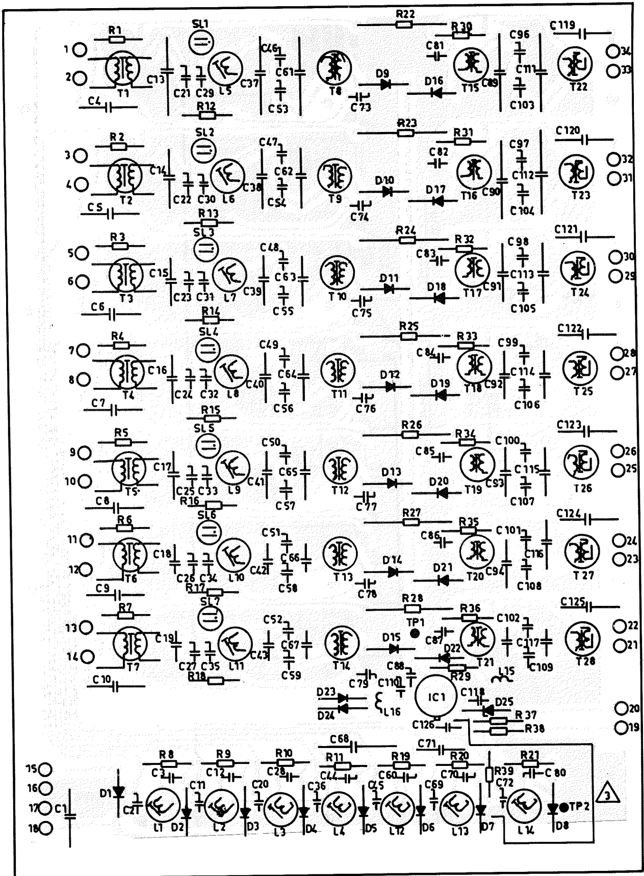
PRINTED CIRCUIT BOARD VIEWED FROM COMPONENT SIDE
