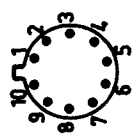
TAA 300 (BOTTOM VIEW)
