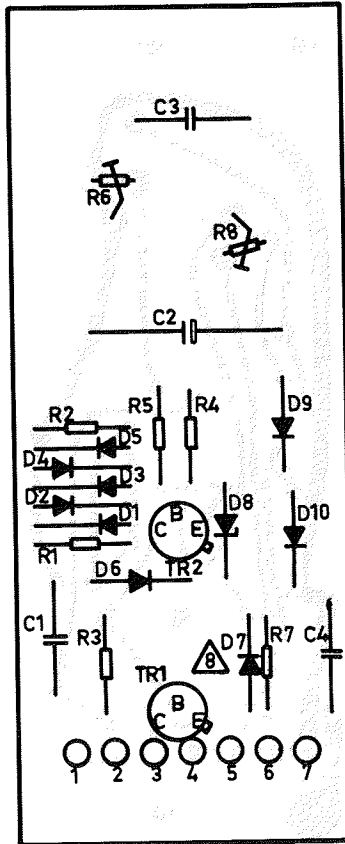
PRINTED CIRCUIT BOARD VIEWED FROM COMPONENT SIDE
