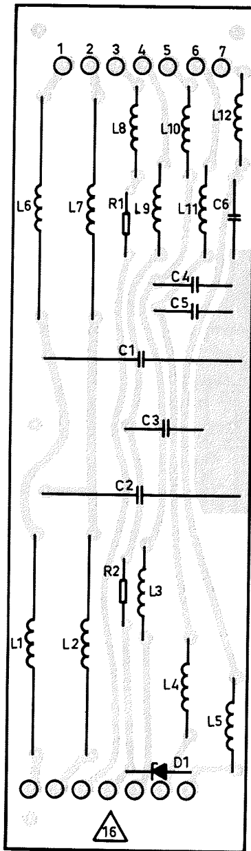
PRINTED CIRCUIT BOARD VIEWED FROM COMPONENT SIDE
